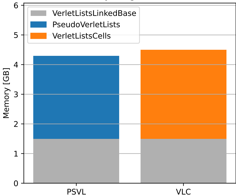
Memory usage (stacked)
