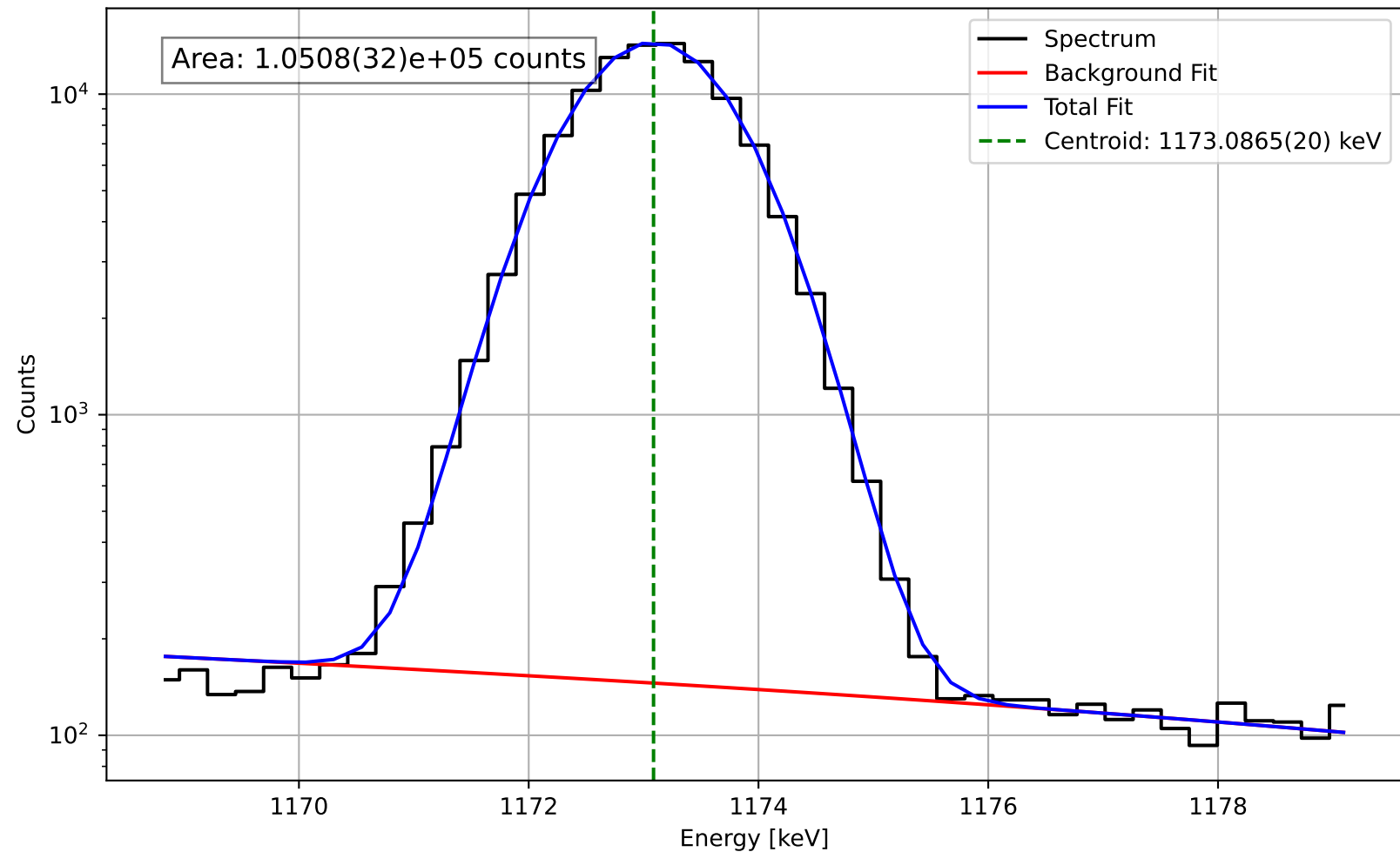
Peak fit for: level-2.cnf at 1173.0865(20) keV
