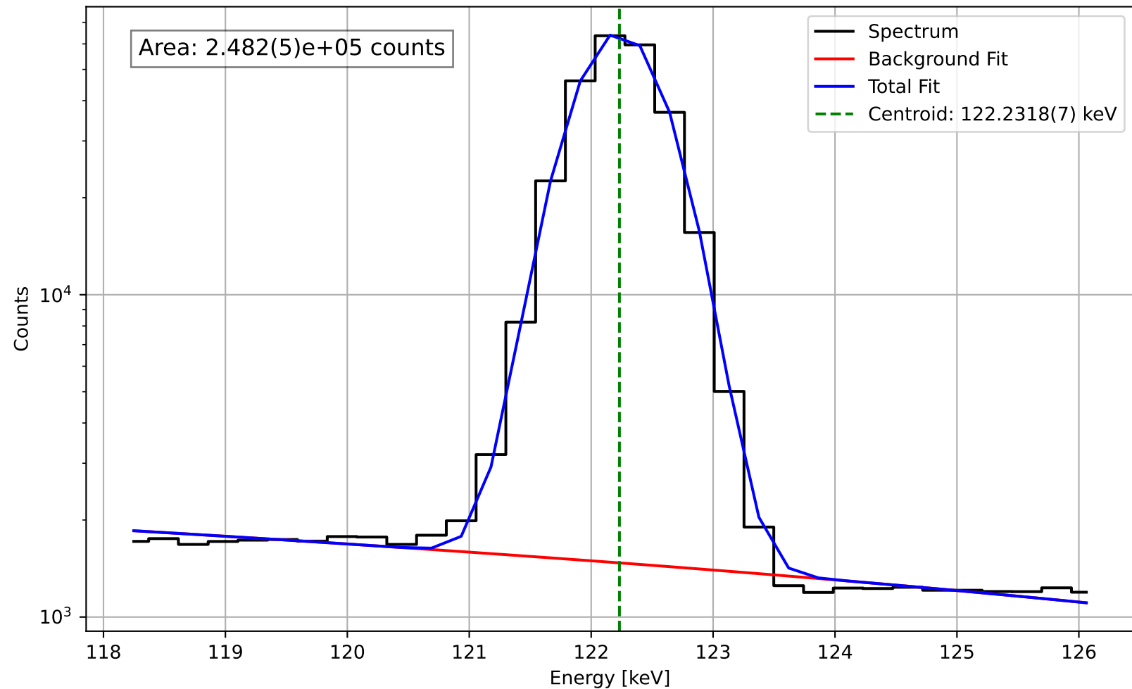
Peak fit for: level-2.cnf at 122.2318(7) keV
