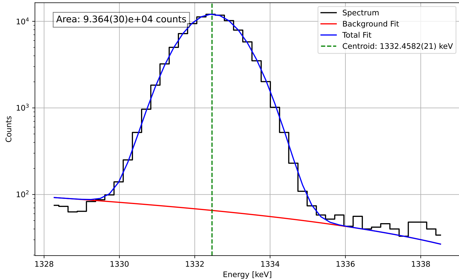
Peak fit for: level-2.cnf at 1332.4582(21) keV
