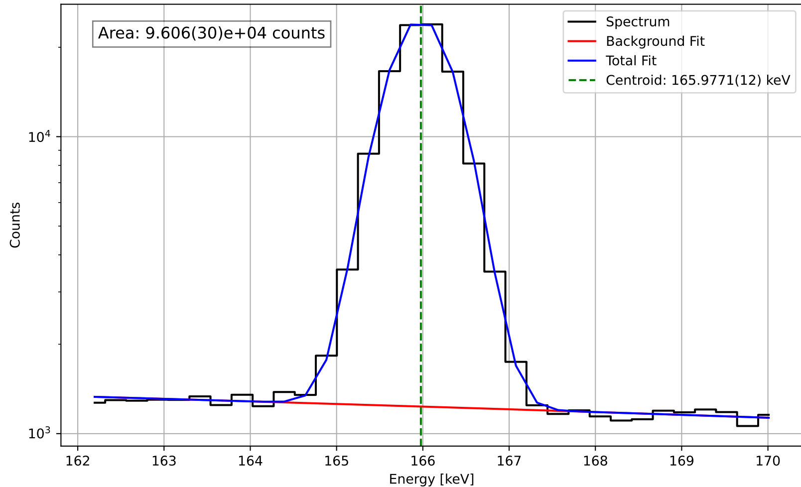
Peak fit for: level-2.cnf at 165.9771(12) keV
