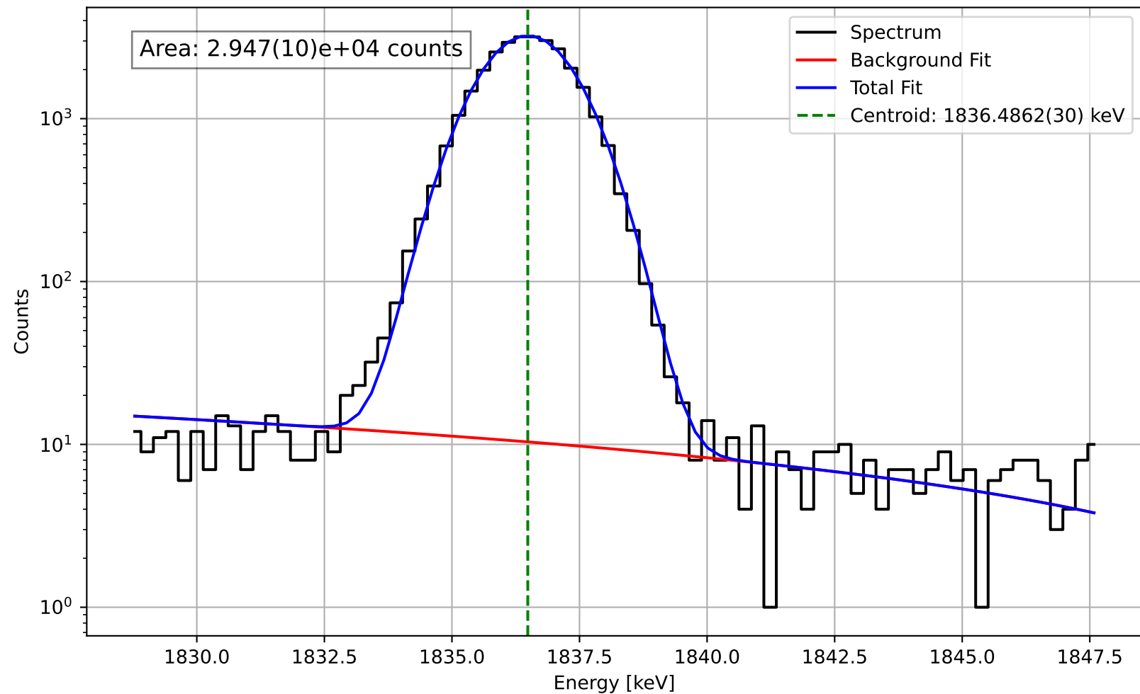
Peak fit for: level-2.cnf at 1836.4862(30) keV
