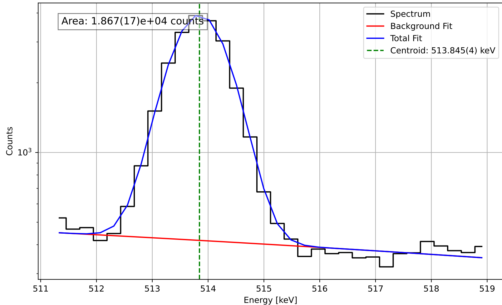
Peak fit for: level-2.cnf at 513.845(4) keV
