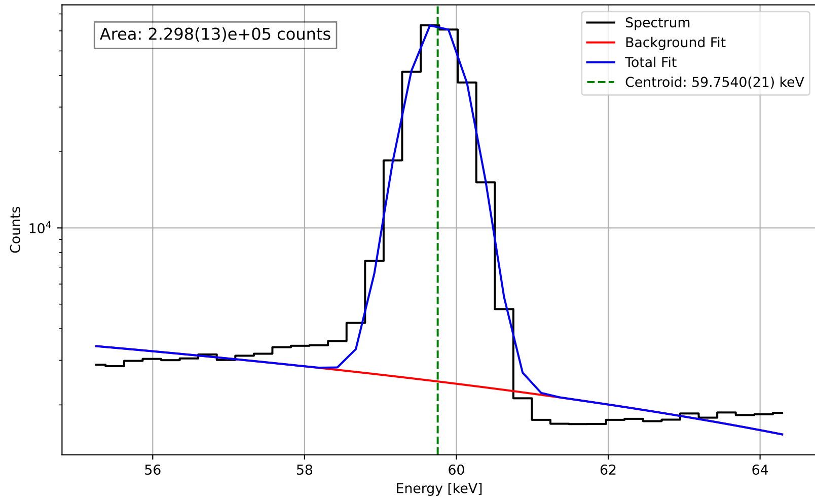
Peak fit for: level-2.cnf at 59.7540(21) keV
