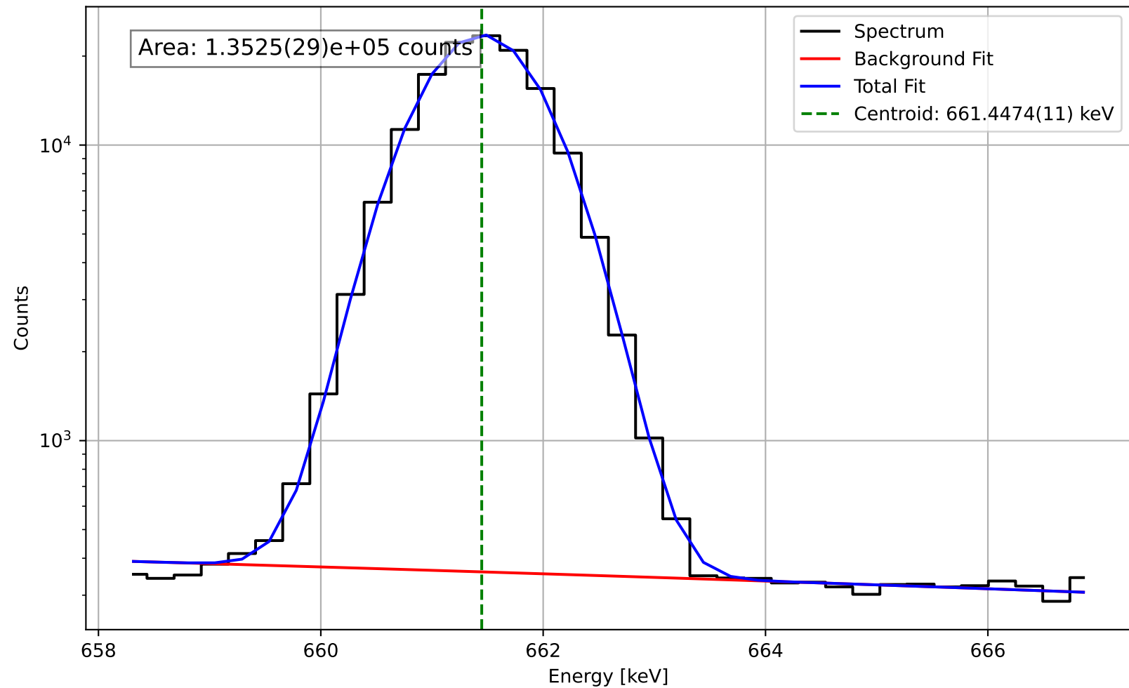
Peak fit for: level-2.cnf at 661.4474(11) keV
