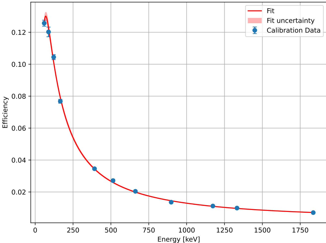
HPGe Detector Efficiency Fit, level 1, with aluminum foil: False
