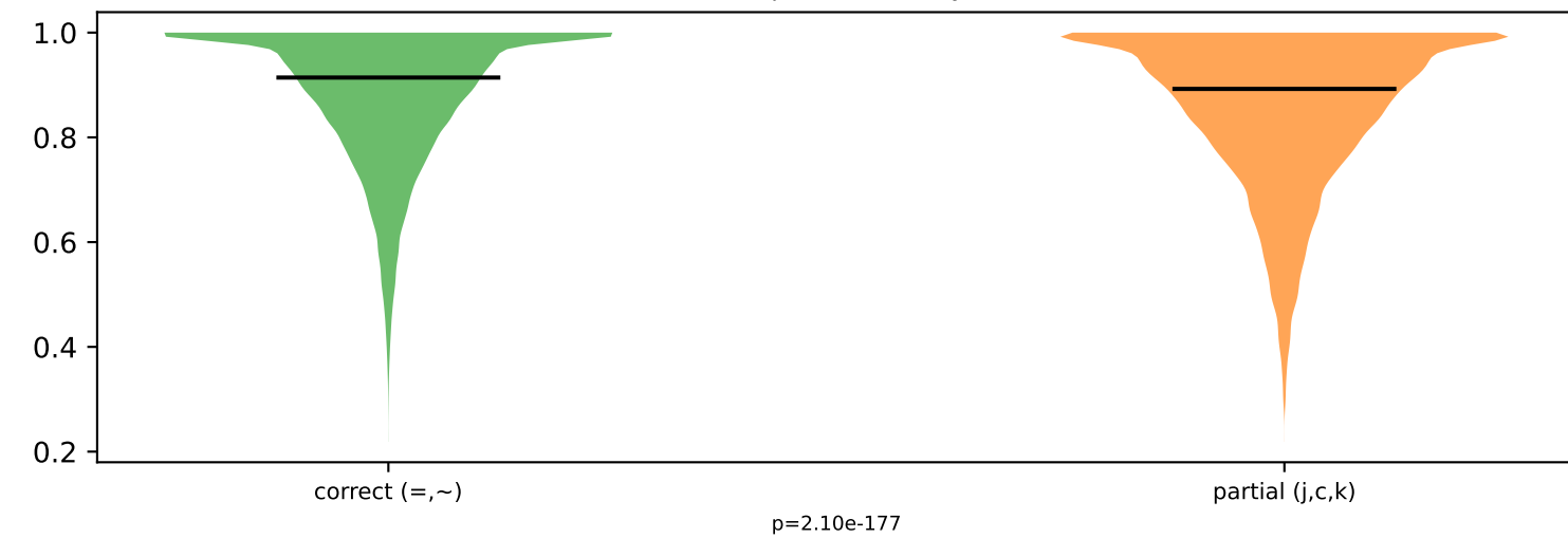
Best target coverage
