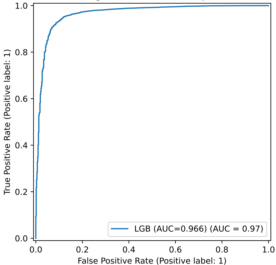
LightGBM ROC — test split
