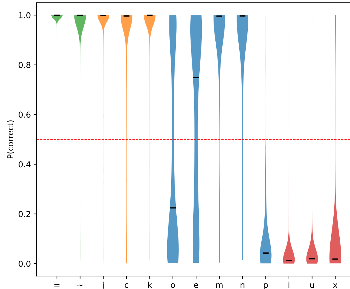
Score distribution per class
