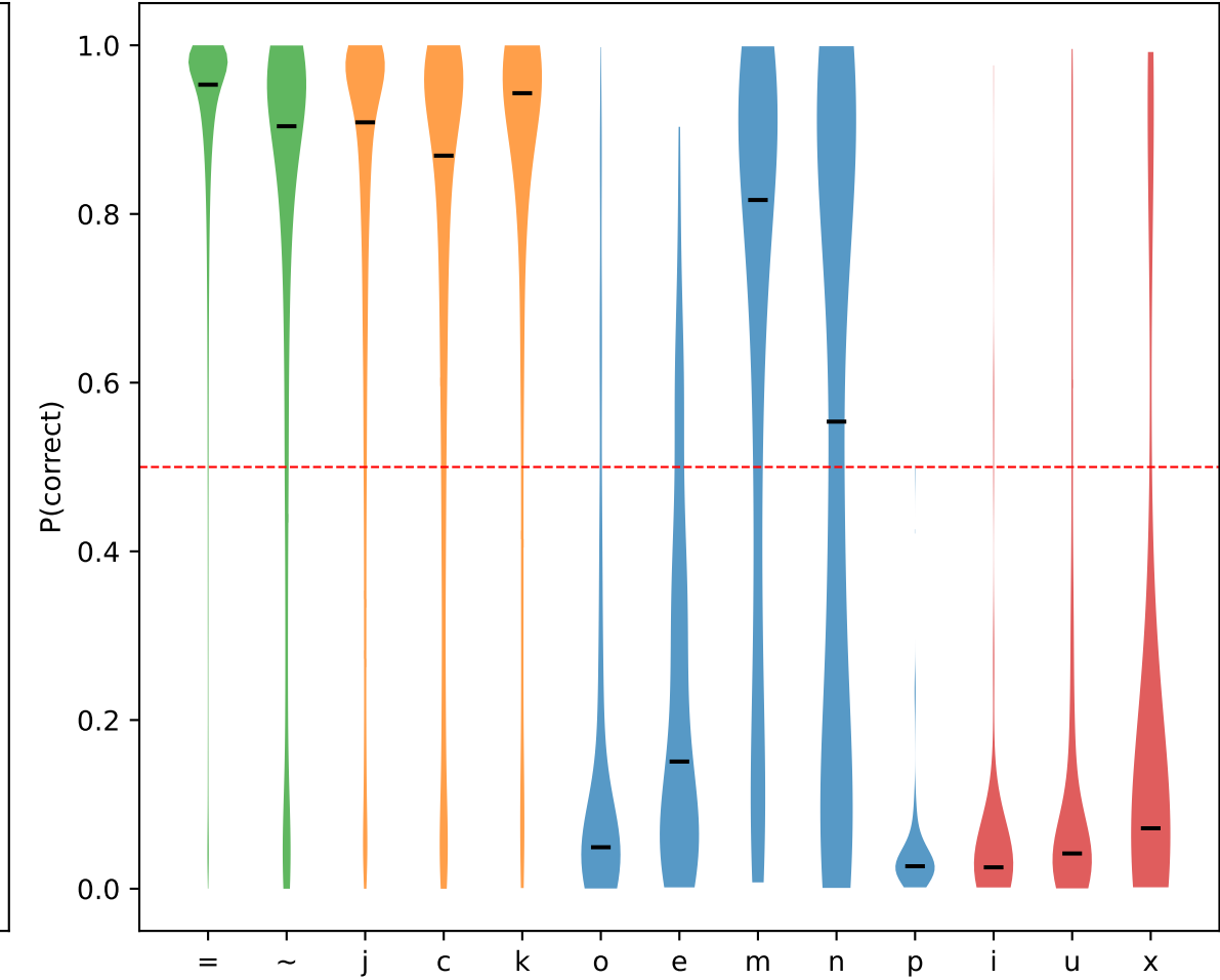
Score distribution per class
