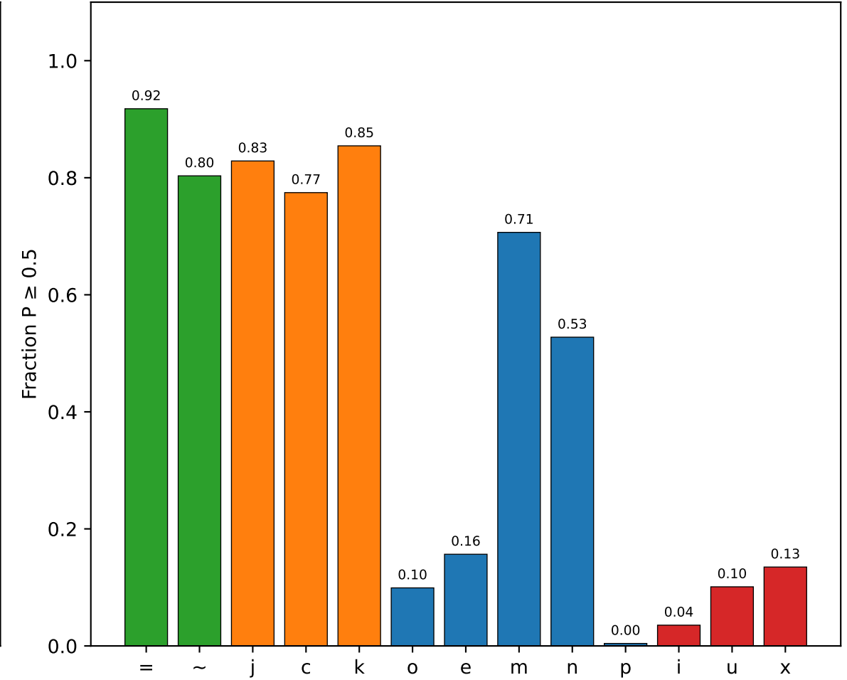
Fraction rescued at P≥0.5
