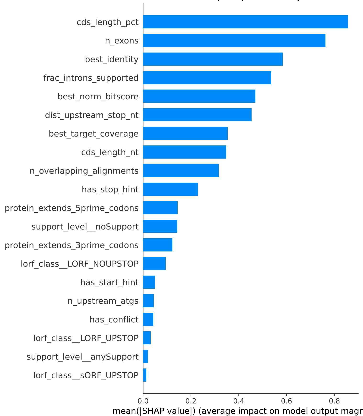
SHAP mean |value| — feature importance
