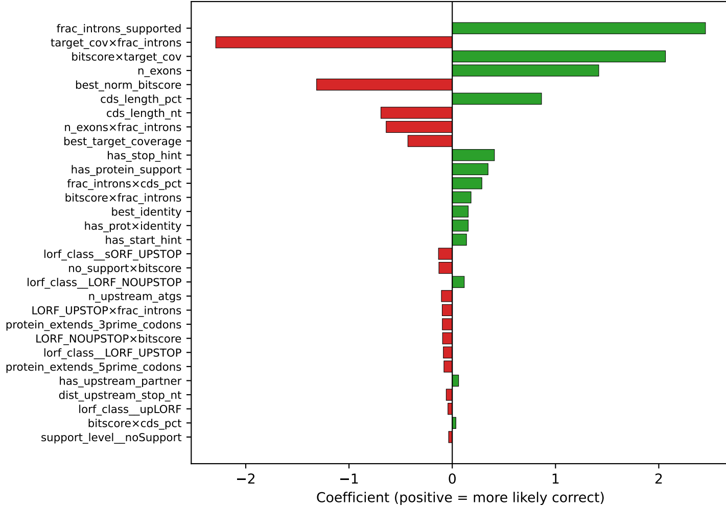
Top-30 coefficients (green=correct, red=wrong)
