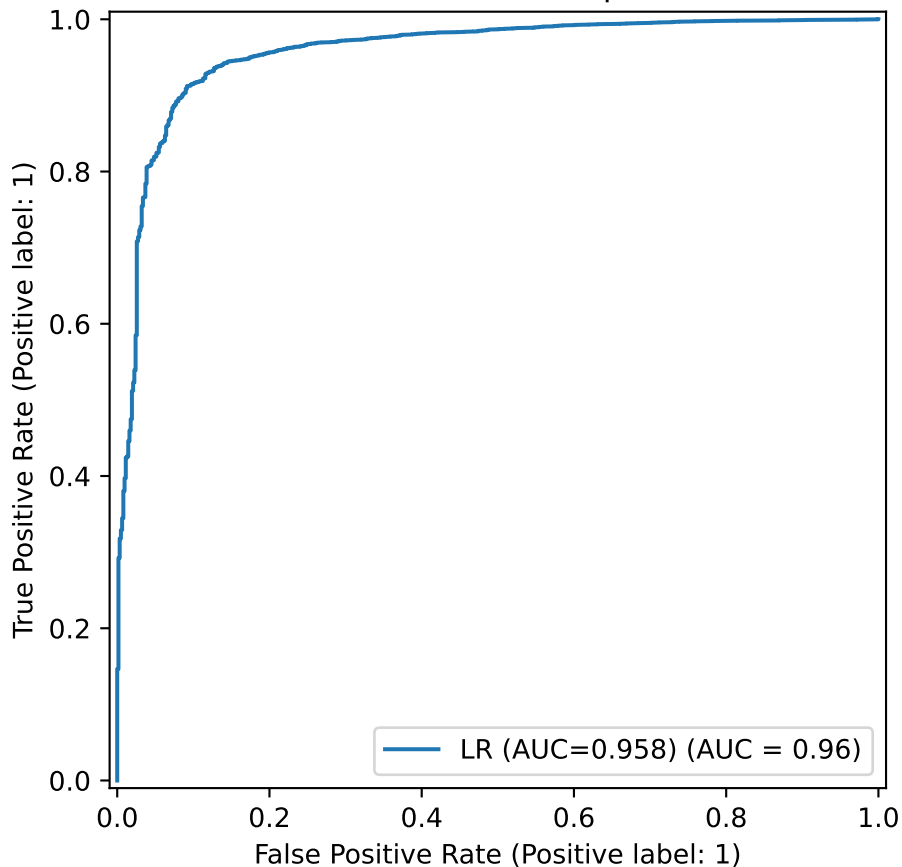
LR ROC — test split
