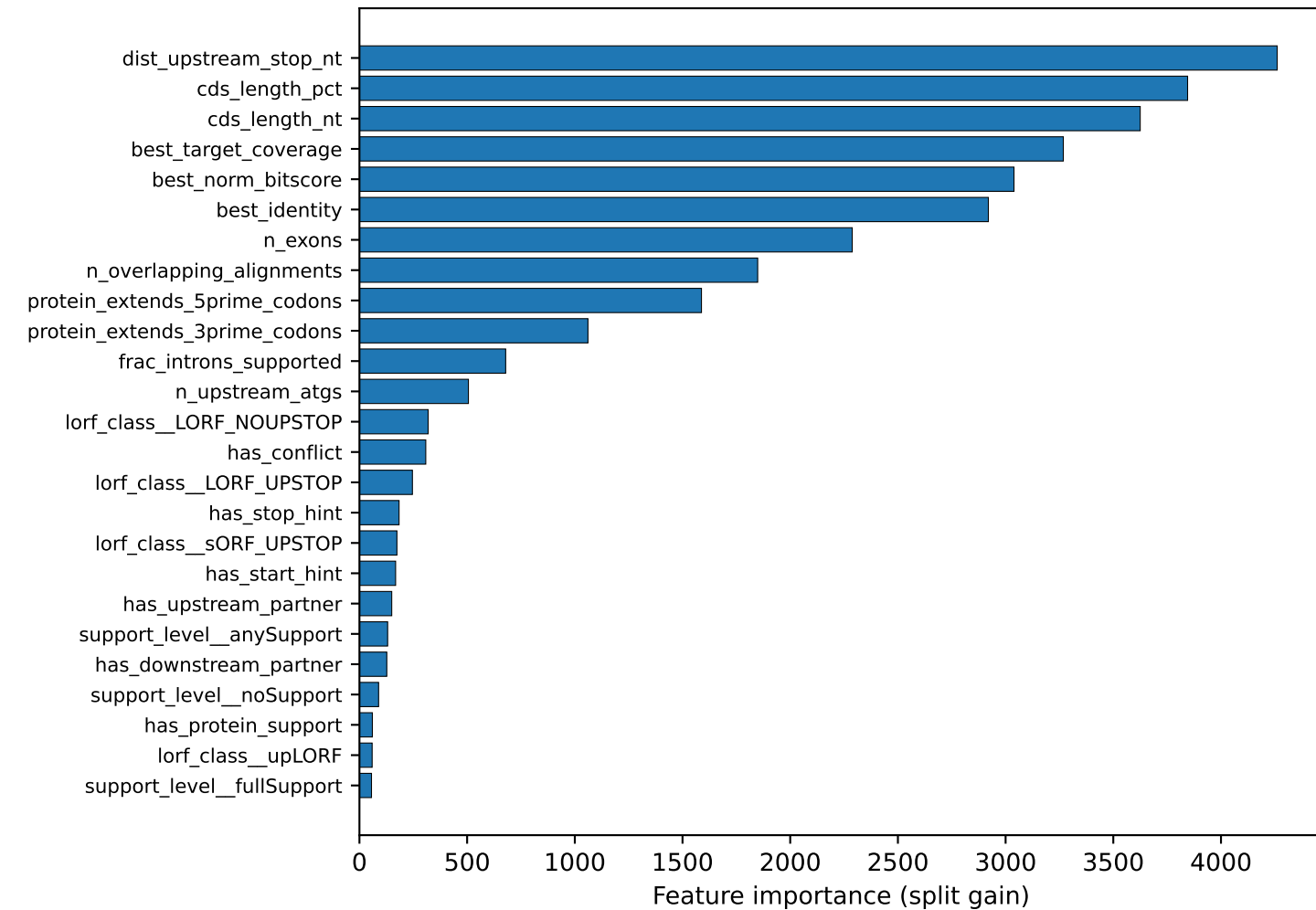
Top-25 features
