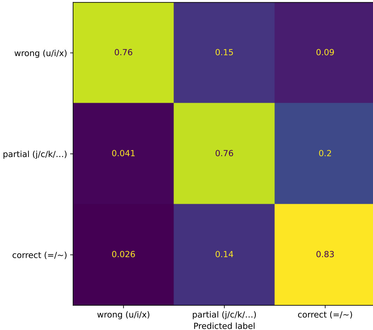
Confusion matrix (row-normalised, test split)
