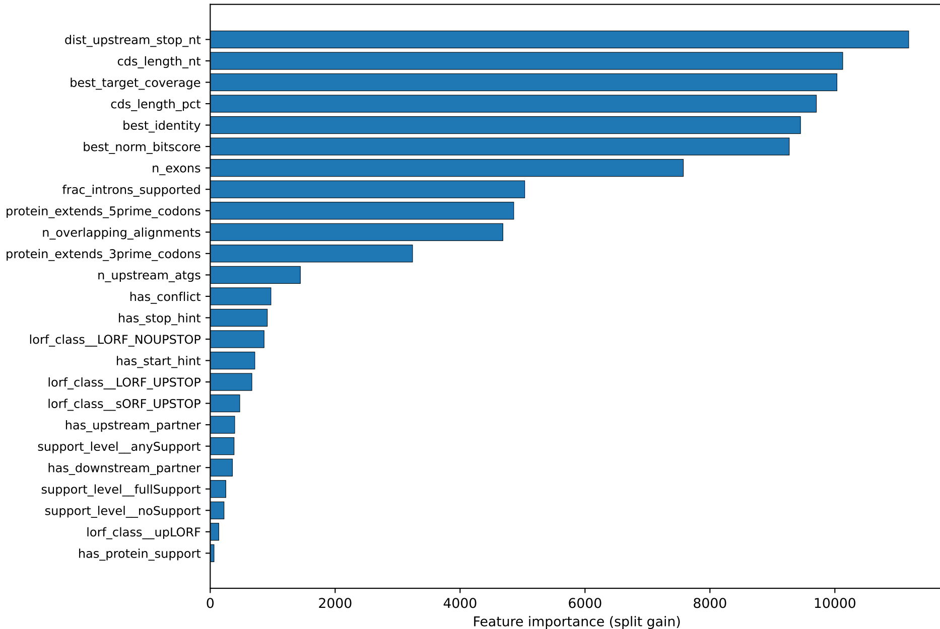
Top-25 features — 3-class LGB
