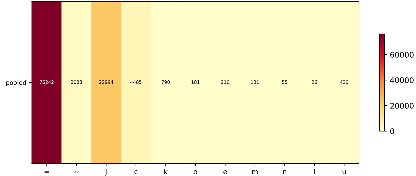
# transcripts
