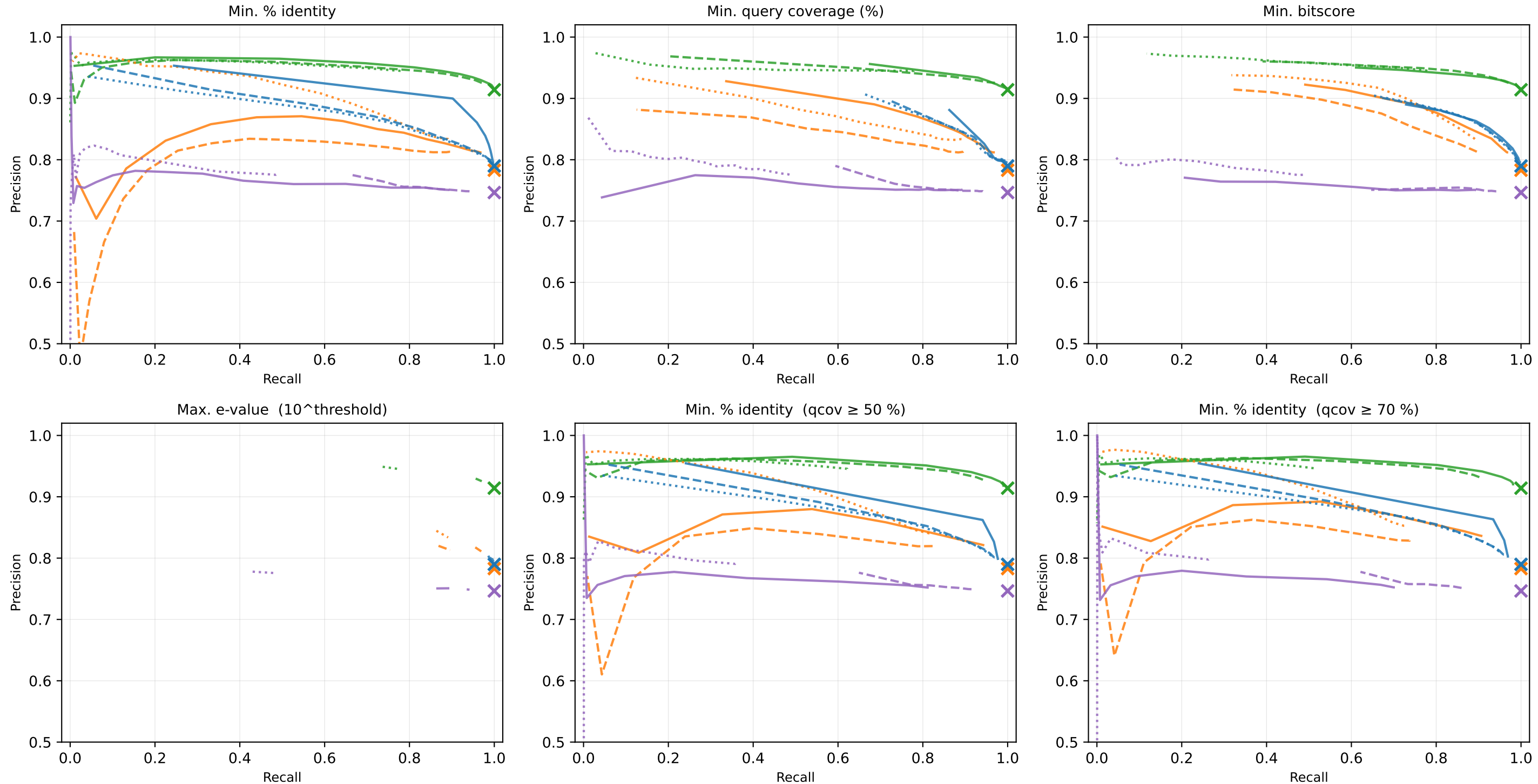
Precision - Recall under Diamond filter rules (lines = ODB exclusion level; × = no-filter baseline)
