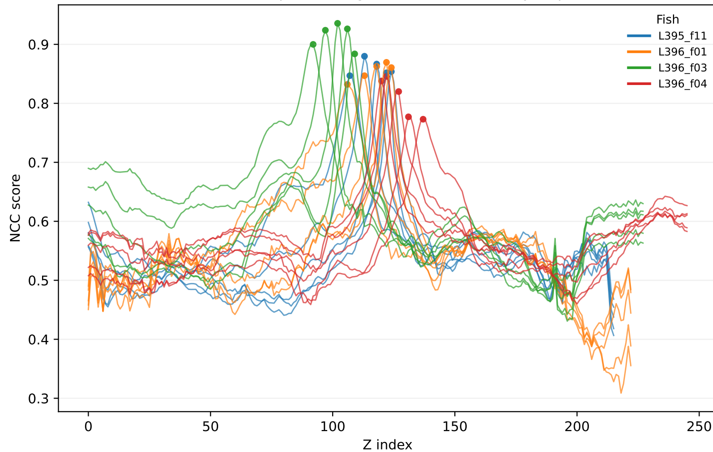
Functional ROIs stay close to their anatomy matches
