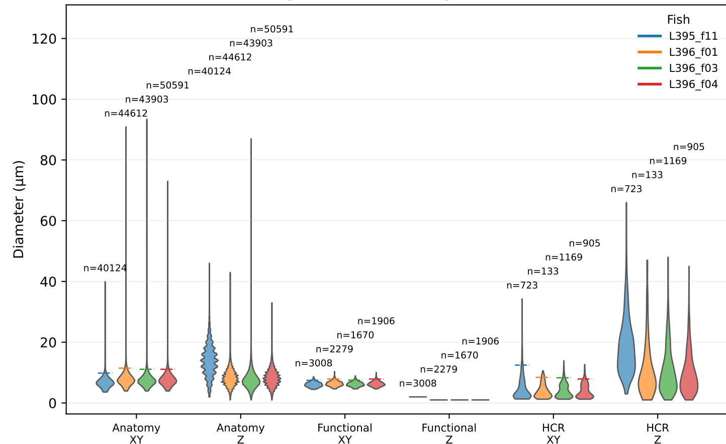
Mask sizes agree across anatomy, function, and HCR
