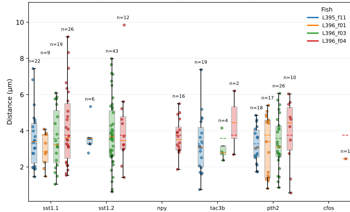
In-plane HCR labels stay close to anatomy matches
