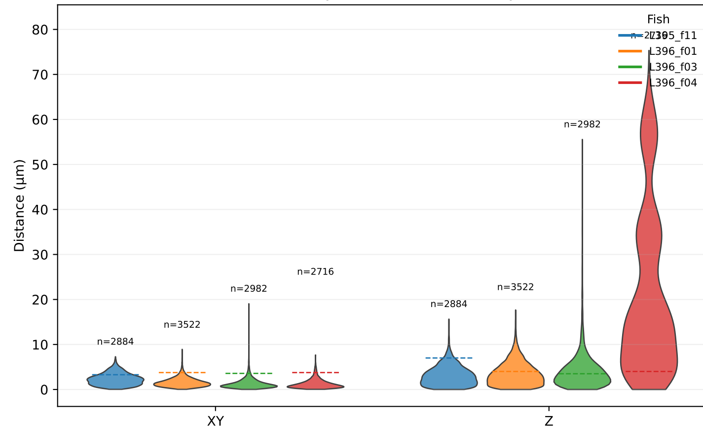
Functional ROIs stay close to their anatomy matches
