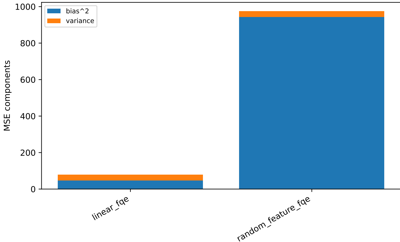
Bias-variance decomposition
