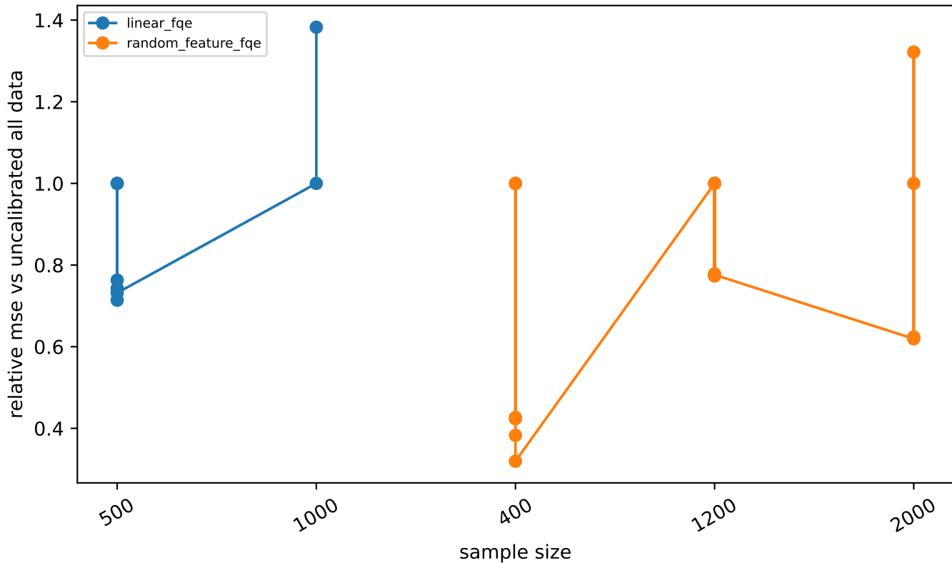
Relative MSE versus sample size
