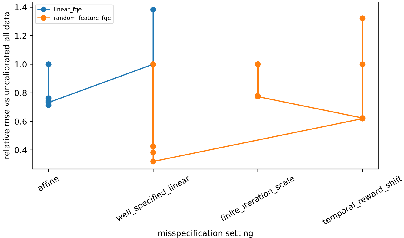
Misspecification/distortion sweep
