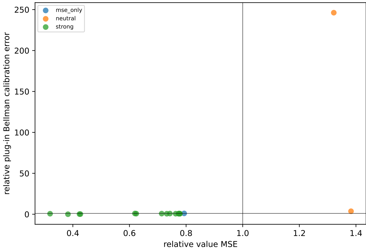
MSE and calibration-error improvement
