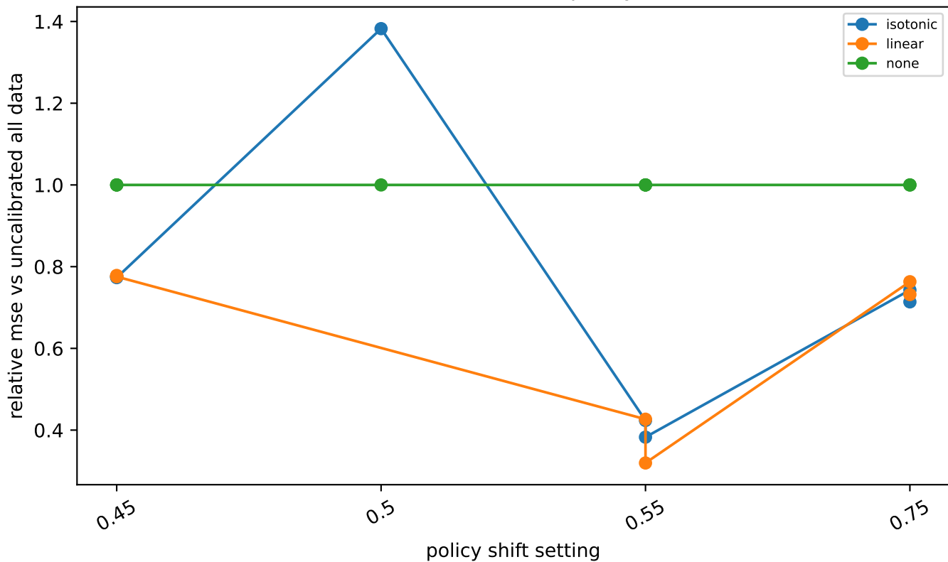
Relative MSE versus policy shift
