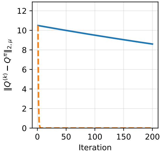
Iteration Curves at \alpha = 0.05
