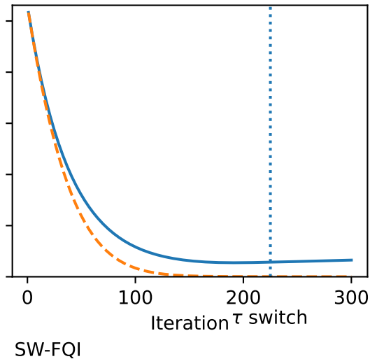
Temperature homotopy
