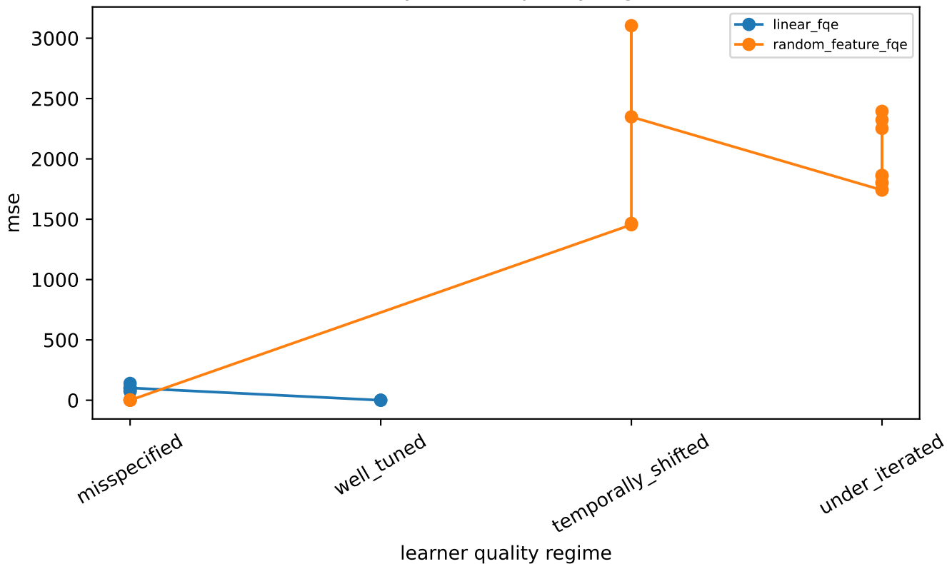
MSE by learner-quality regime
