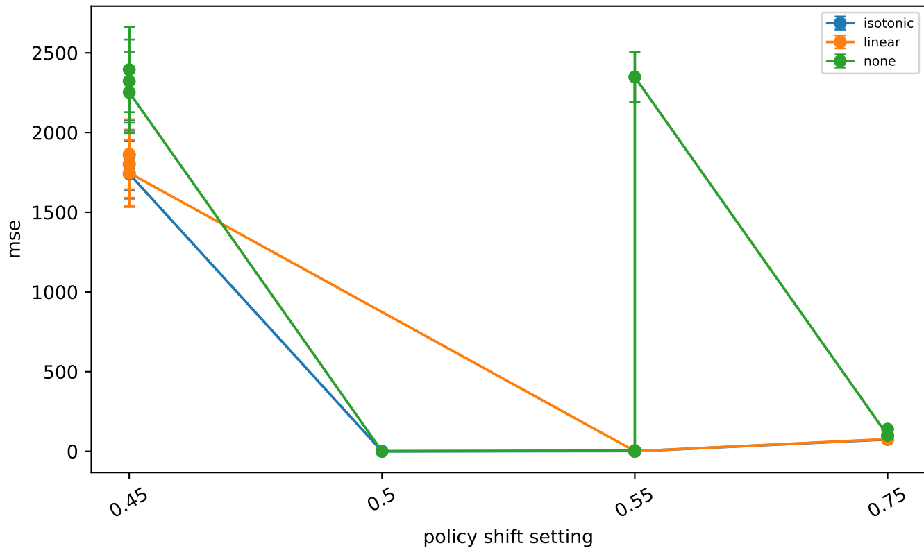
MSE versus policy shift
