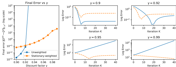
(b) Garnet: high-discount instability.
