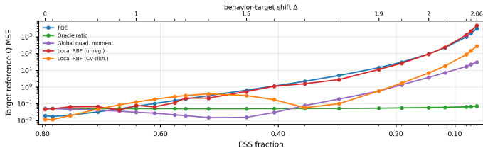
(c) Controlled benchmark: target-reference Q error.
