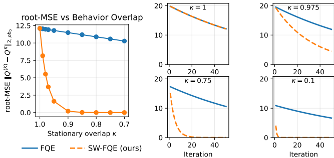
(a) Baird: overlap controls contraction.
