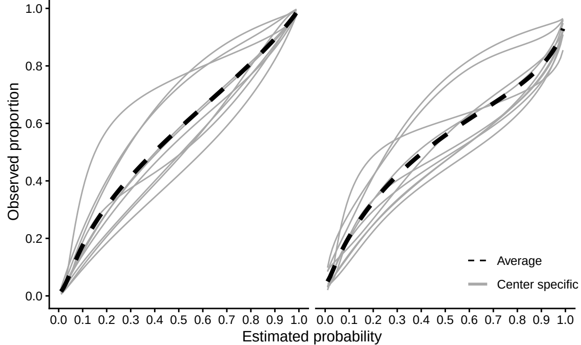
Logistic regression
