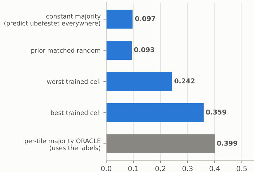
Macro-IoU separates them
