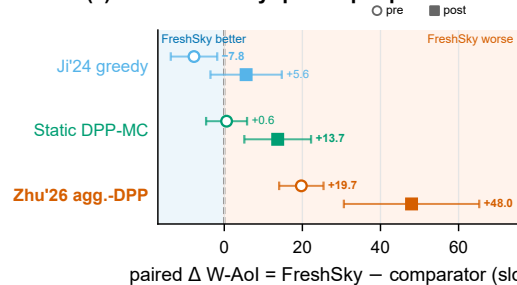
(c) Shift boundary: paired pre/post
