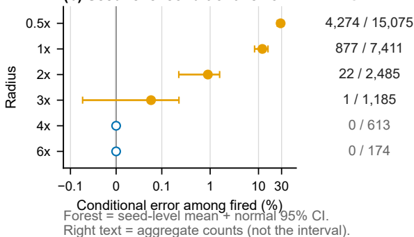
(b) Seed-level conditional error
