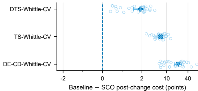
(b) Paired 30-seed effects (95% intervals)
