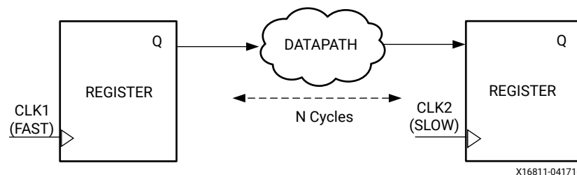
Figure 77: Multicycles Between FAST-to-SLOW Clocks
