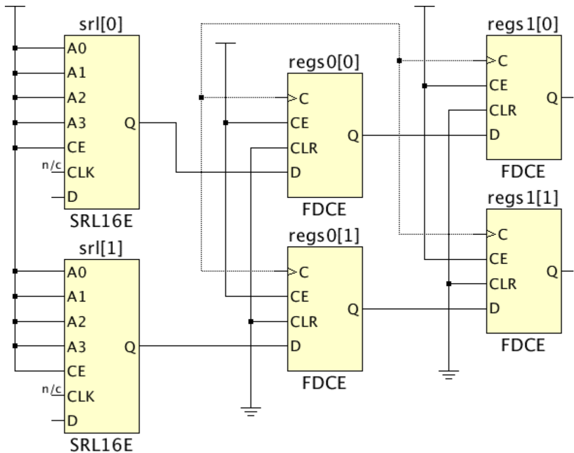
Figure 100: Schematic of Example Circuit
