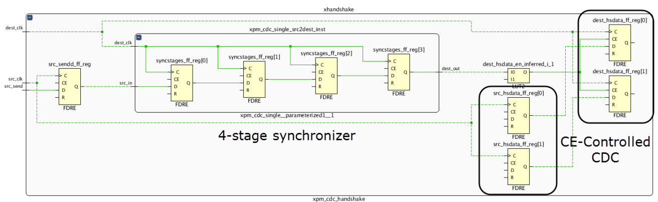
Figure 93: set_bus_skew Example One
