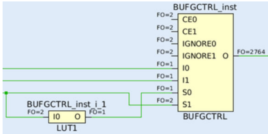
Figure 91: Netlist Before Optimization
