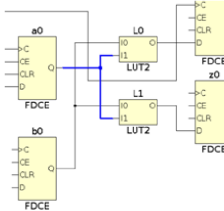
Figure 97: Simple Design to Illustrate Routing Constraints
