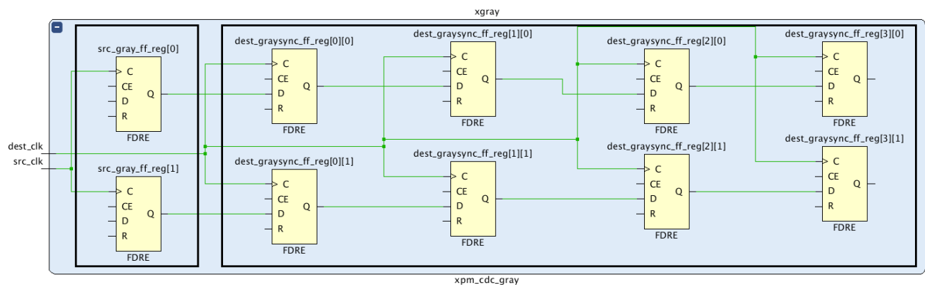
Figure 94: set_bus_skew Example Two
