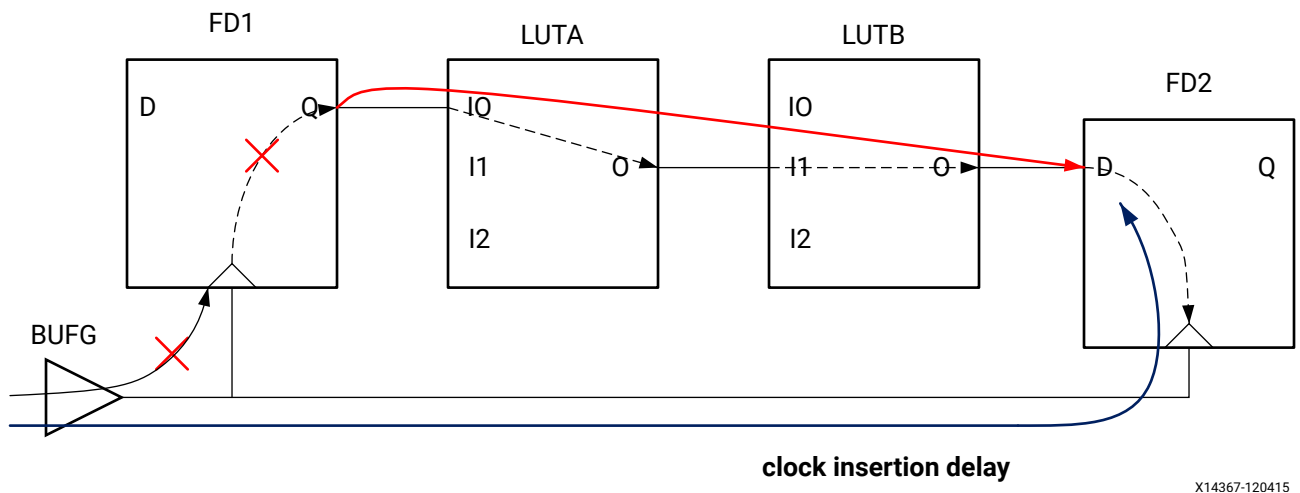
Figure 86: Path Segmentation Result in Large Skew
