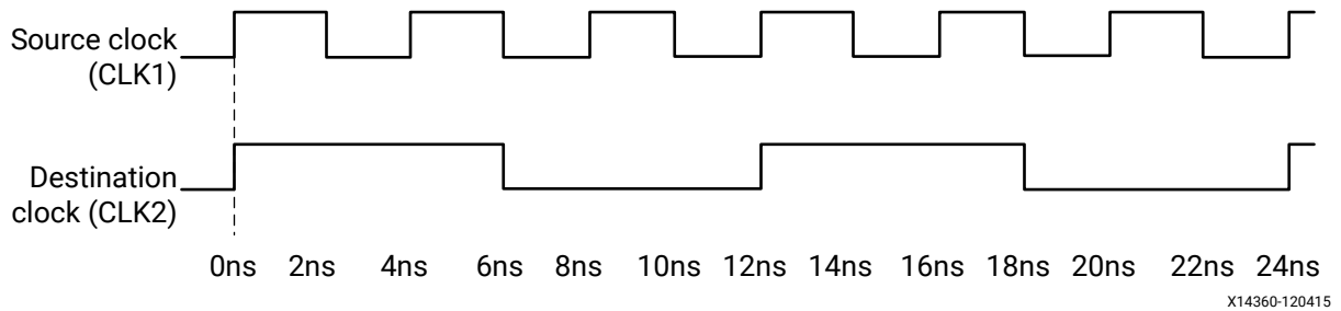
Figure 78: Multicycles Between FAST-to-SLOW Clocks
