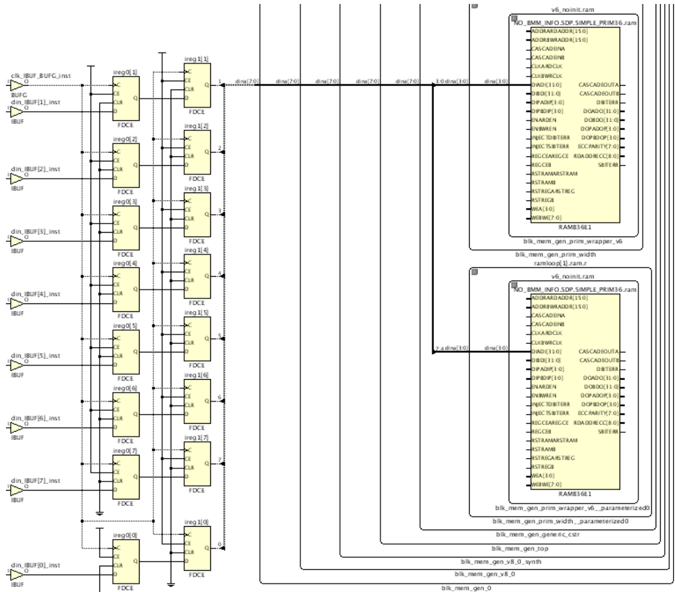
Figure 102: Example Circuit for Absolute Grid
