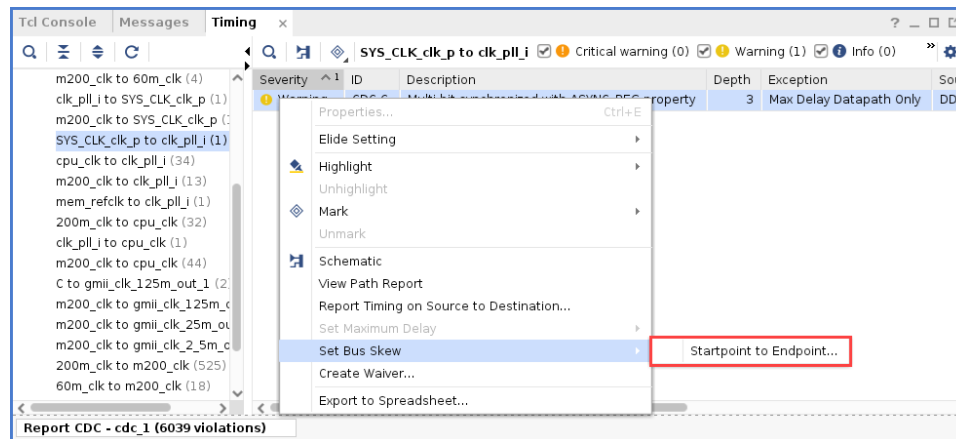
Figure 95: Setting Bus Skew within Report CDC
