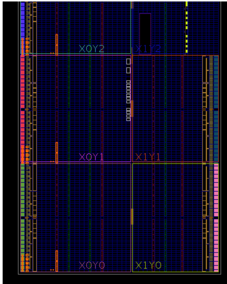
Figure 104: Three Possible Locations for the XDC Macro
