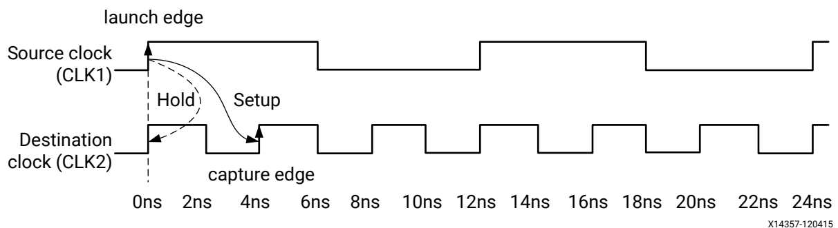
Figure 74: Default Setup and Hold Relationships
