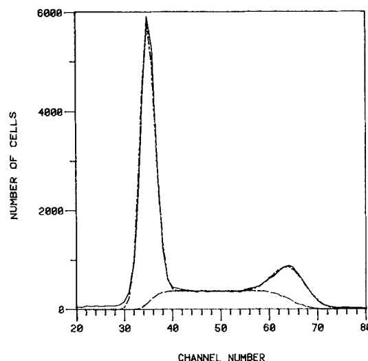
FIG. 1. Flow cytometry data obtained from an asynchronous HeLa cell population and analyzed by the model. The solid line connects the actual data values. (-----) is the total fit by the model to the data. (----) is the S-phase portion of the total fit to the data. This representation also applies for Figures 2 and 3. A point-by-point subtraction of the S-phase curve from the total fit would yield the normal curves which represent the G_1 and G_2 + M peaks.
