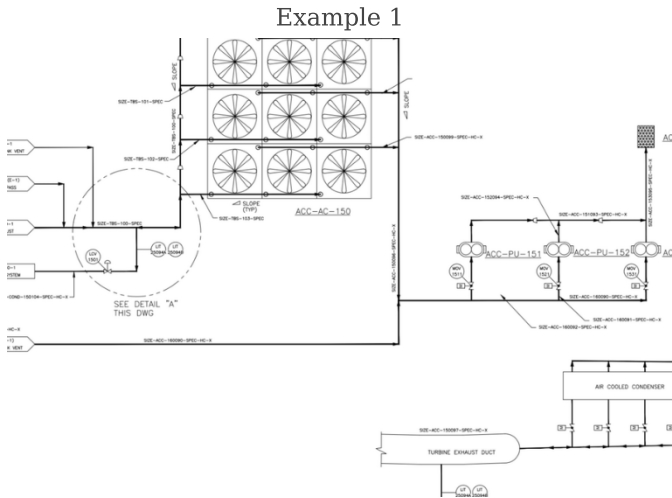
Real P&ID (OPEN100)
