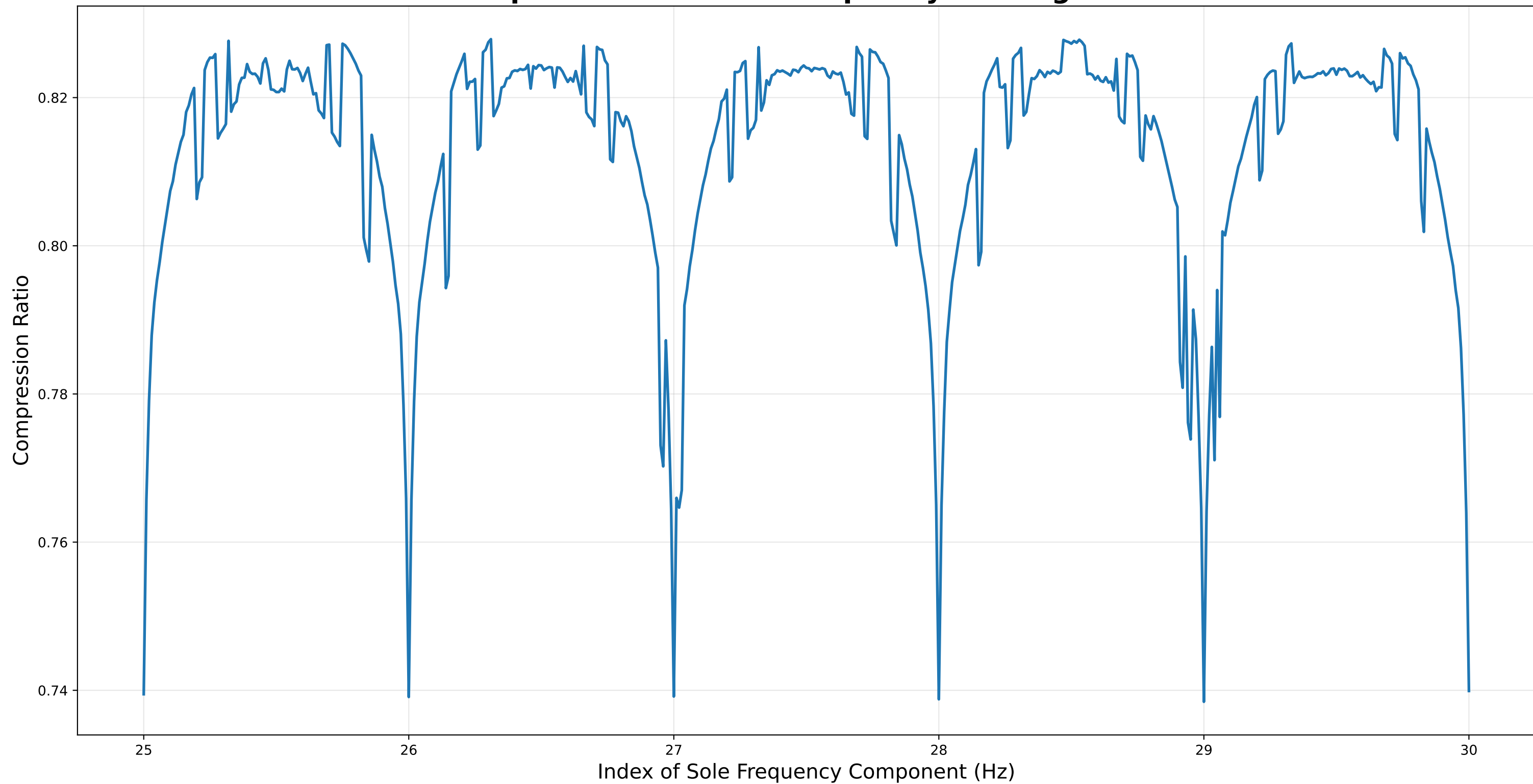
Compression Ratio vs Frequency Bin Alignment
