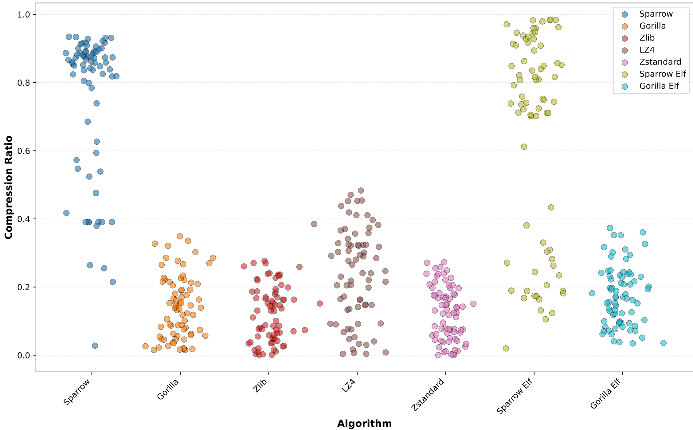
Compression Ratios Across All Datasets (lower is better)
