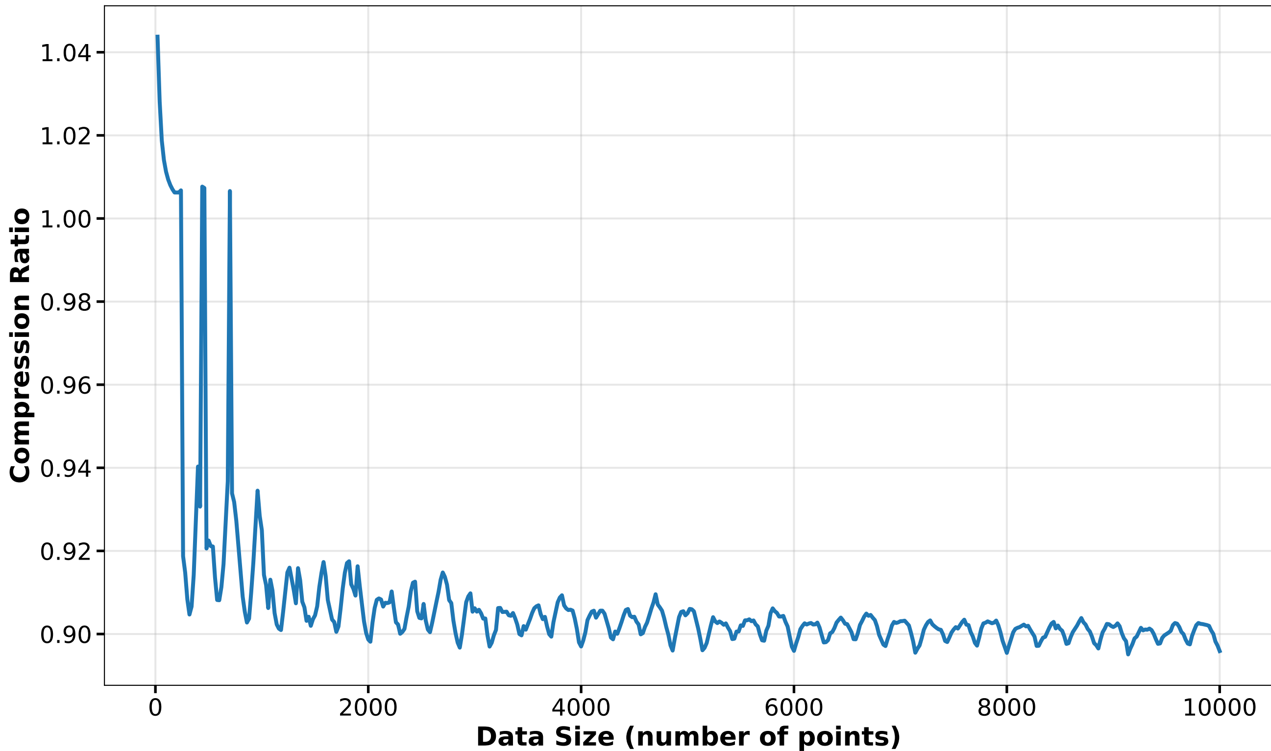
Compression Ratio vs Data Size
