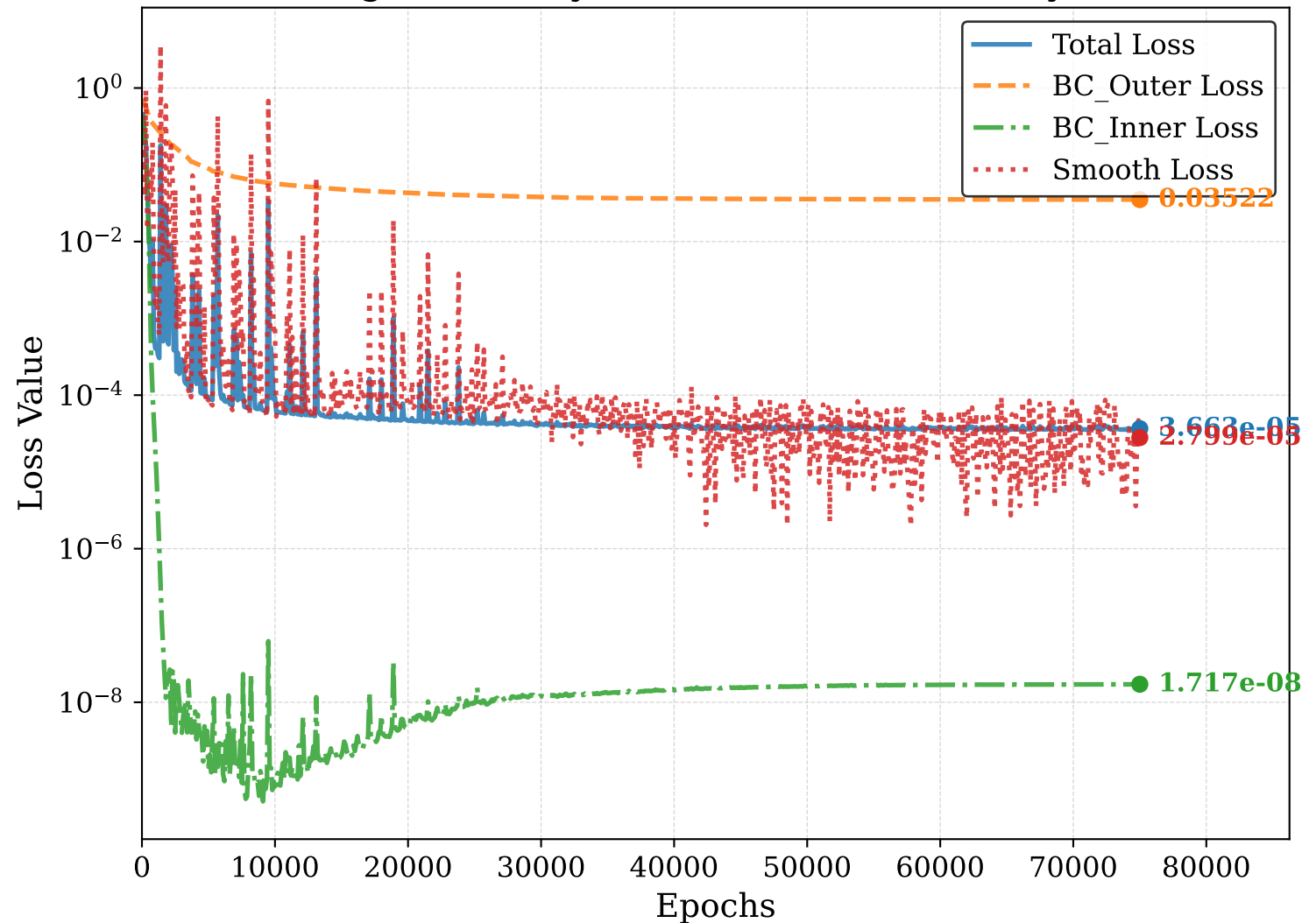
Convergence Analysis of Different Boundary Losses
