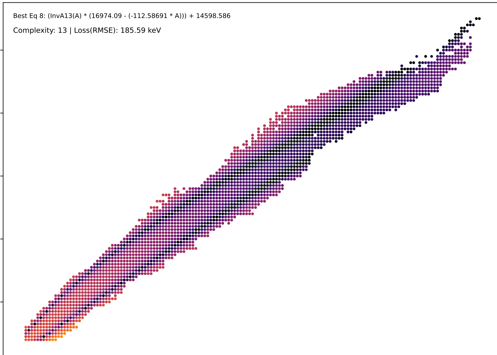
Chart of Nuclides - PySR B vs SEMF per nucleon - Absolute Error
