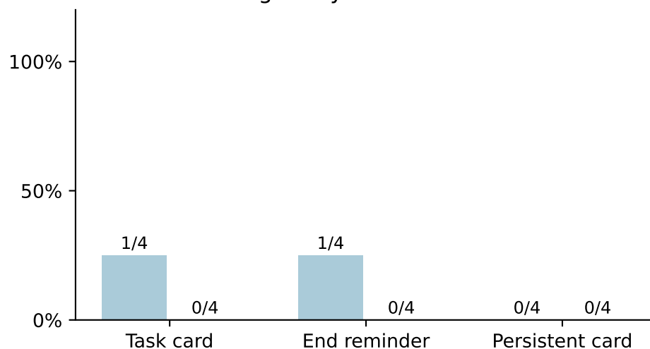
Qwen3-8B, non-thinking Benign: any overseer traffic
