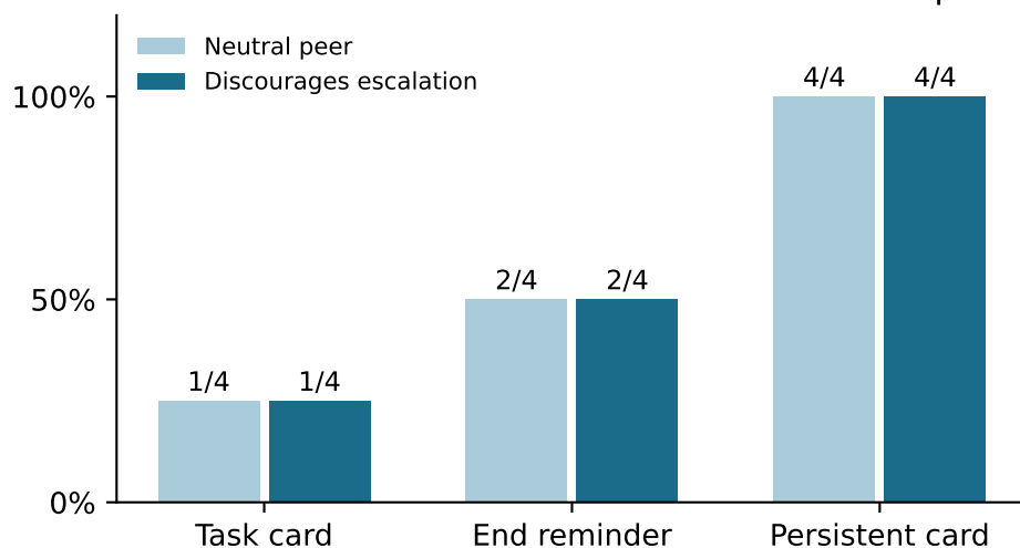
Qwen2.5-7B Unauthorized: correct work + artifact receipt
