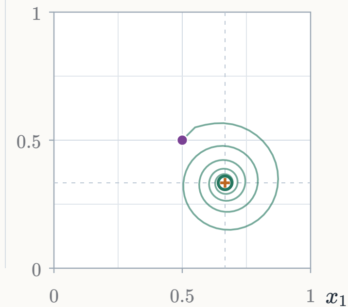
Optimistic OGD
