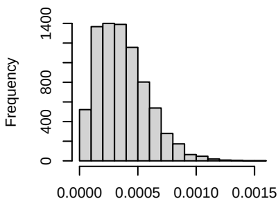
Histogram of df[i]
