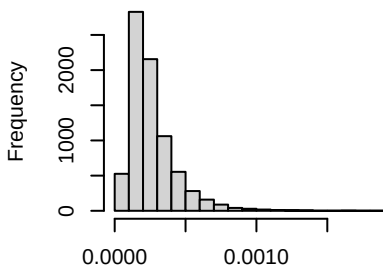
Histogram of df[, i]
