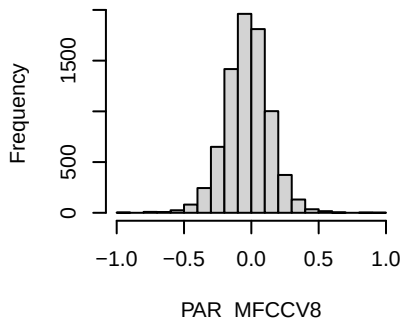
Histogram of df[i]
