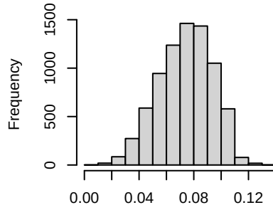
Histogram of df[i]
