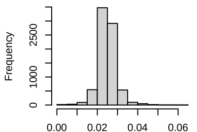
Histogram of df[, i]
