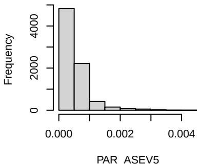
Histogram of df[, i]
