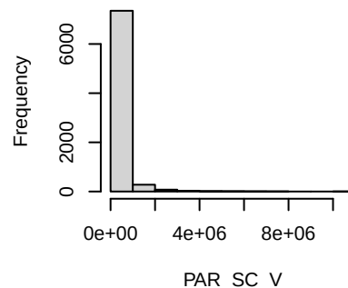
Histogram of df[, i]
