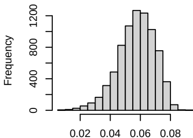
Histogram of df[i]
