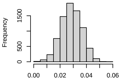
Histogram of df[i]
