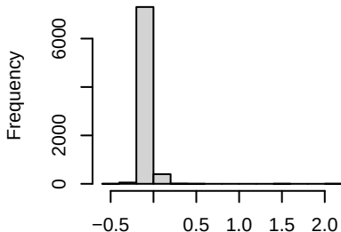
Histogram of df[, i]
