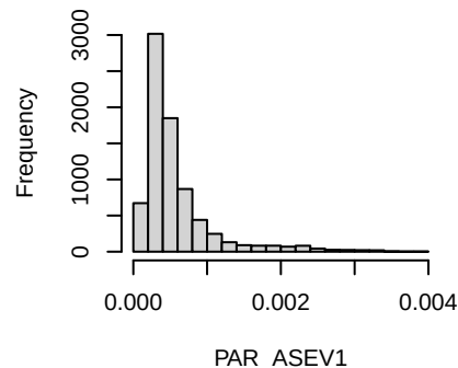
Histogram of df[, i]
