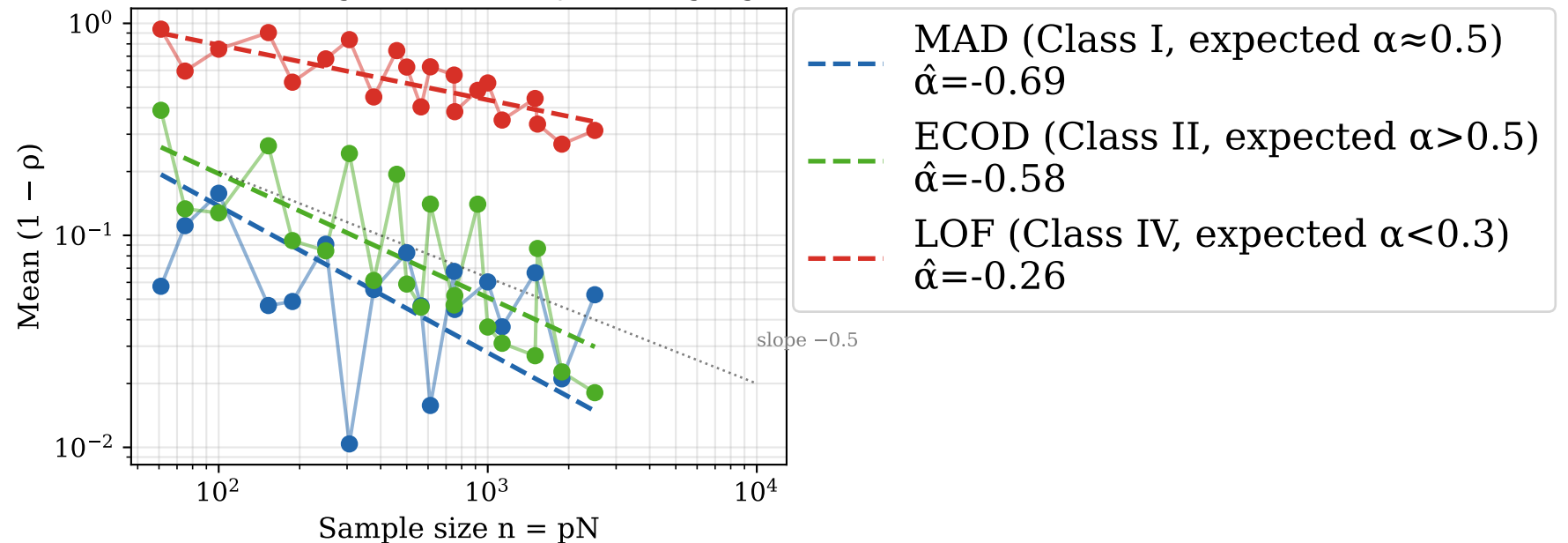
E2 — Convergence Rate: 1-\rho vs n (log-log)
