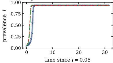
Higher-order SIS
