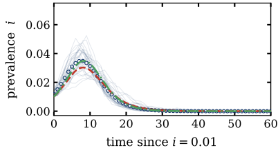
Pairwise SIR
