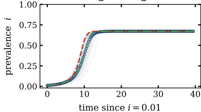
Interacting contagions
