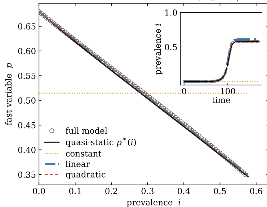
Higher-order (simplicial)
