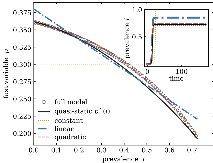
Adaptive network SIS
