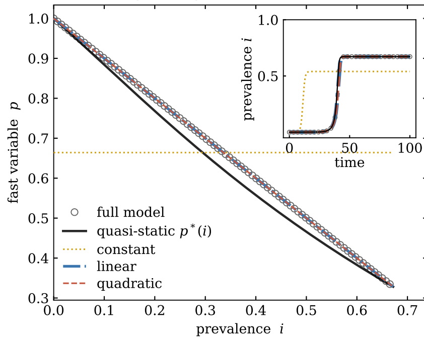
Interacting contagions
