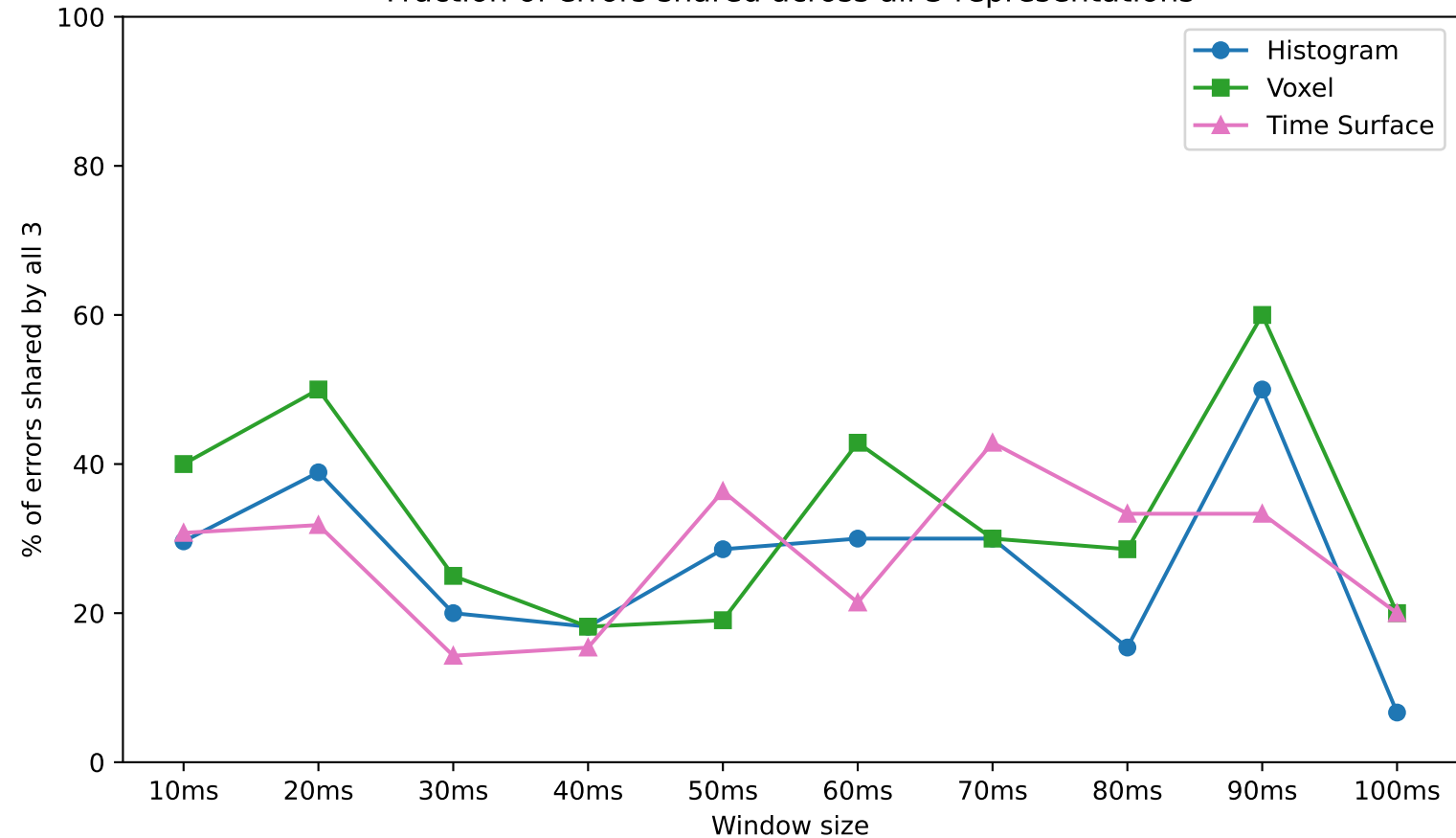
Fraction of errors shared across all 3 representations
