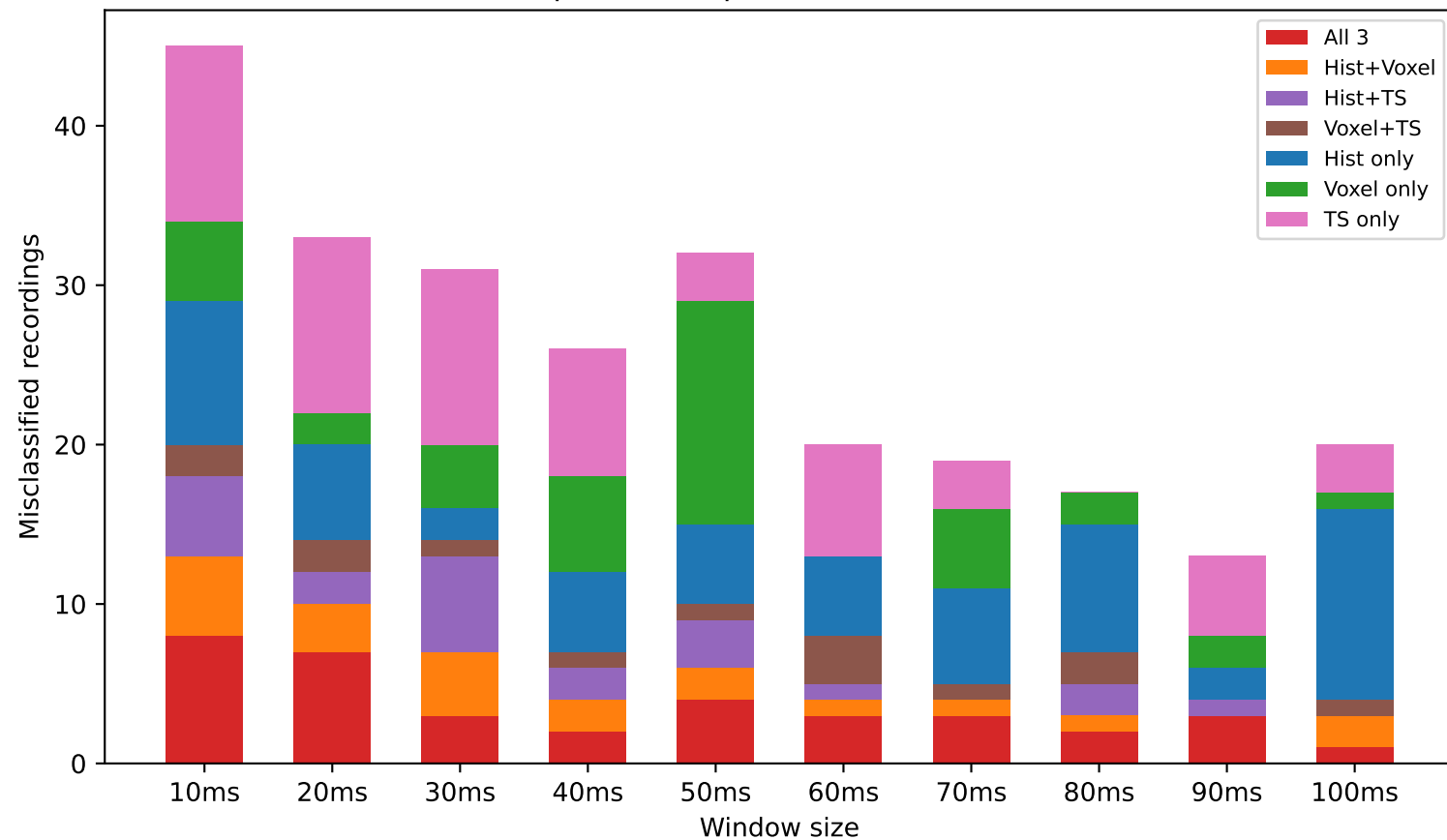
Error overlap across representations (RQ1, offset=0)
