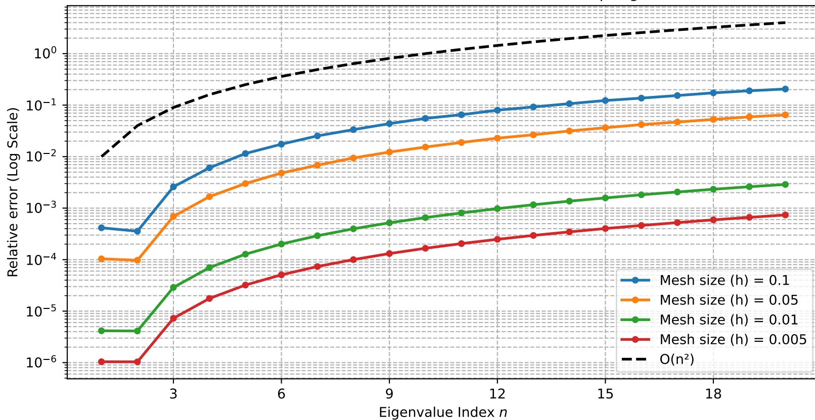
Relative errors between exact and numerical ND map eigenvalues
