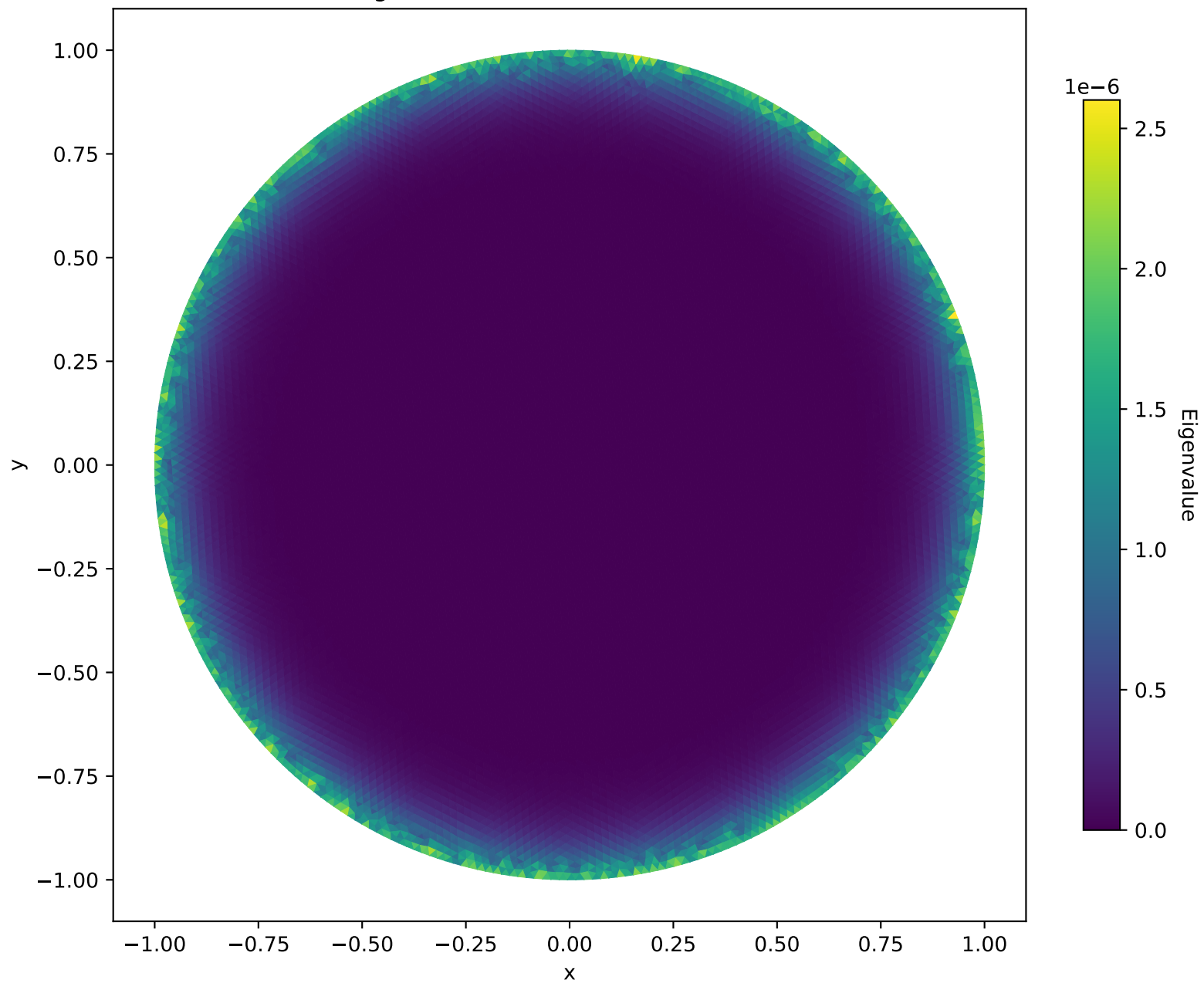
N'th diagonal element of the Frechet derivative
