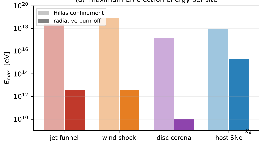
(a) maximum CR-electron energy per site
