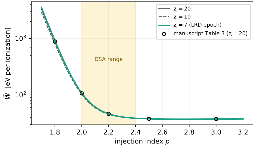
(b) energy per ionization for a power-law injection
