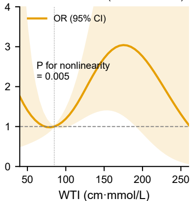
B CHARLS 2011 (cross-sectional)
