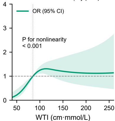
C CHARLS 2011-2018 (7-y prospective)
