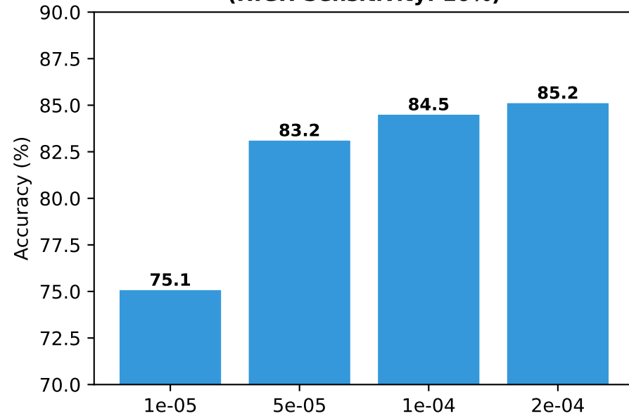
Learning Rate (HIGH Sensitivity: 10%)
