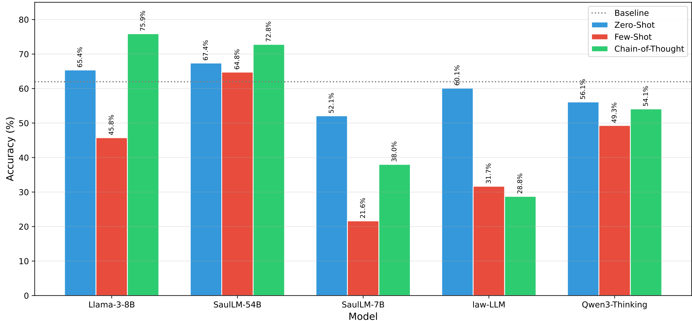
Prompting Strategy Comparison Across Models
